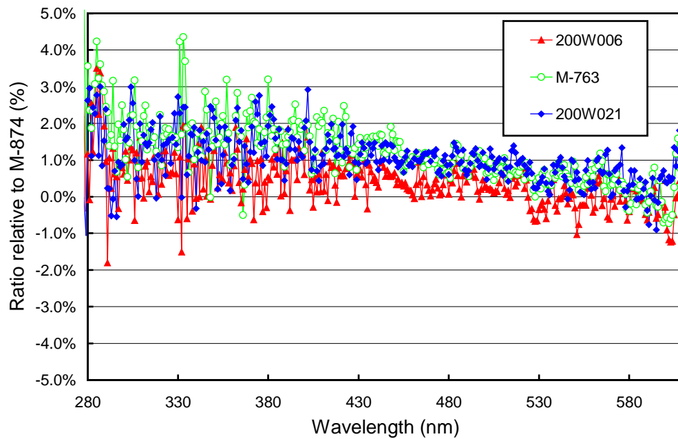
Figure 5.3.2. Comparison of South Pole lamps 200W006, M-763, and 200W021 with the BSI traveling standard M-874 at the end of the season on 1/13/99.
