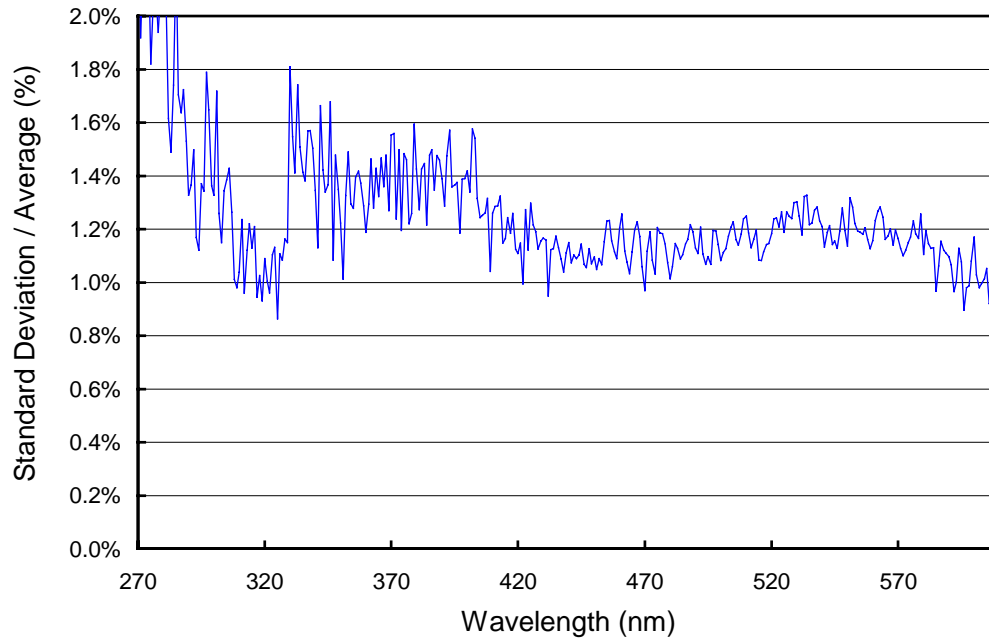
Figure 5.3.4. Ratio of standard deviation and average calculated from the absolute calibration scans of the South Pole 1998-99 season.
