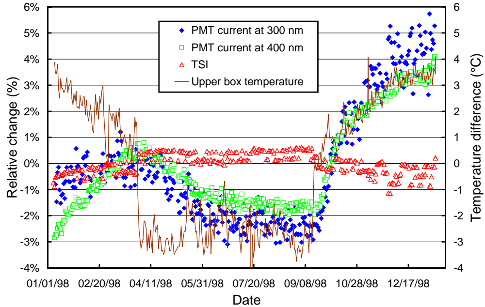
Figure 5.3.3. Time-series of PMT current at 300 and 400 nm, instrument temperature, and TSI signal during measurements of the internal irradiance standard performed during the South Pole 1998-99 season. The data are normalized to the average of the whole period.
