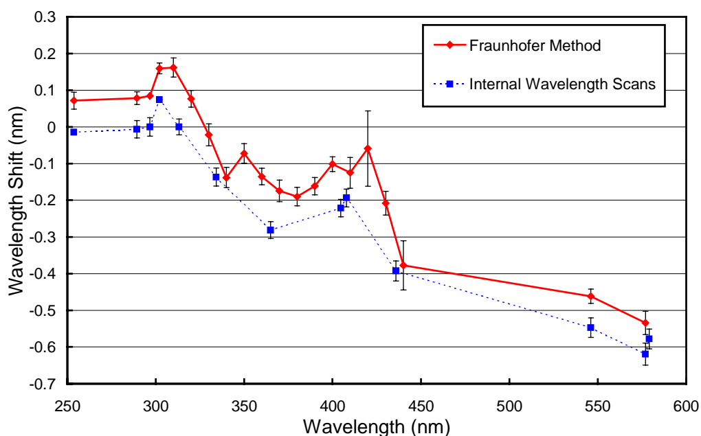
Figure 5.3.6. Monochromator non-linearity for the South Pole 1998-99 season. Thick line: Correction function calculated with the Fraunhofer-correlation method, applied to correct the South Pole Volume 8 data. Thin broken line: Correction function calculated with the method that was historically applied. The offset difference between both methods is 0.08 nm. The error bars show the 1\sigma standard deviation of the wavelength shift for the season.
