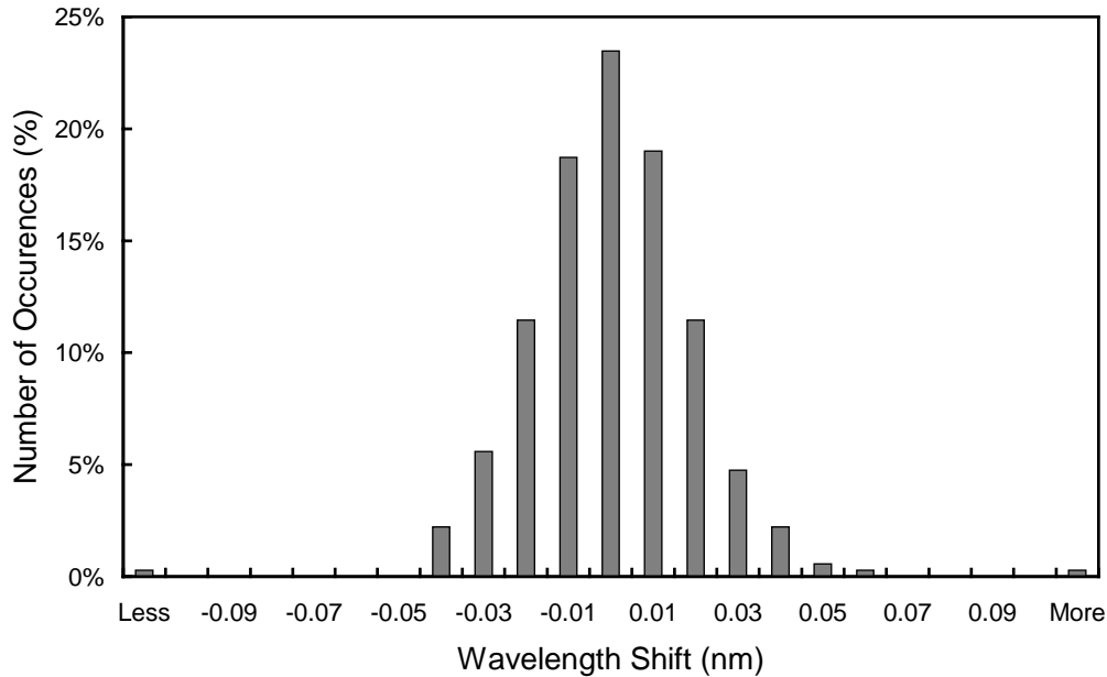
Figure 5.3.5. Differences in the measured position of the 296.73 nm mercury line between consecutive wavelength scans. The x-labels give the center wavelength shift for each column. The 0-nm histogram column covers the range -0.005 to +0.005 nm. “Less” means shifts smaller than -0.105 nm; “more” means shifts larger than 0.105 nm.
