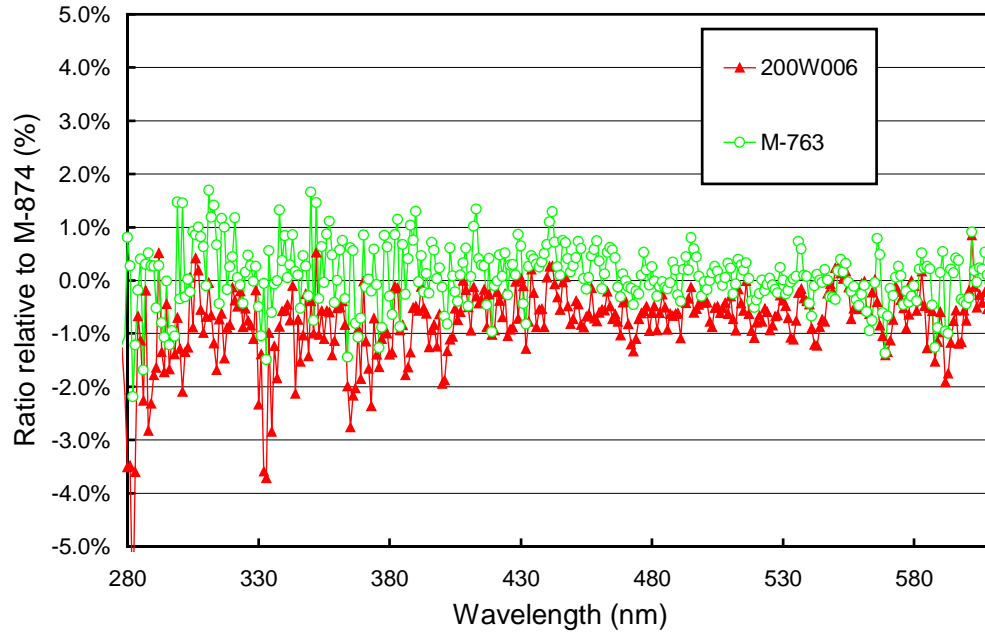
Figure 5.3.1. Comparison of South Pole lamps 200W006 and M-763 with the BSI traveling standard M-874 at the start of the season on 2/7/98.
