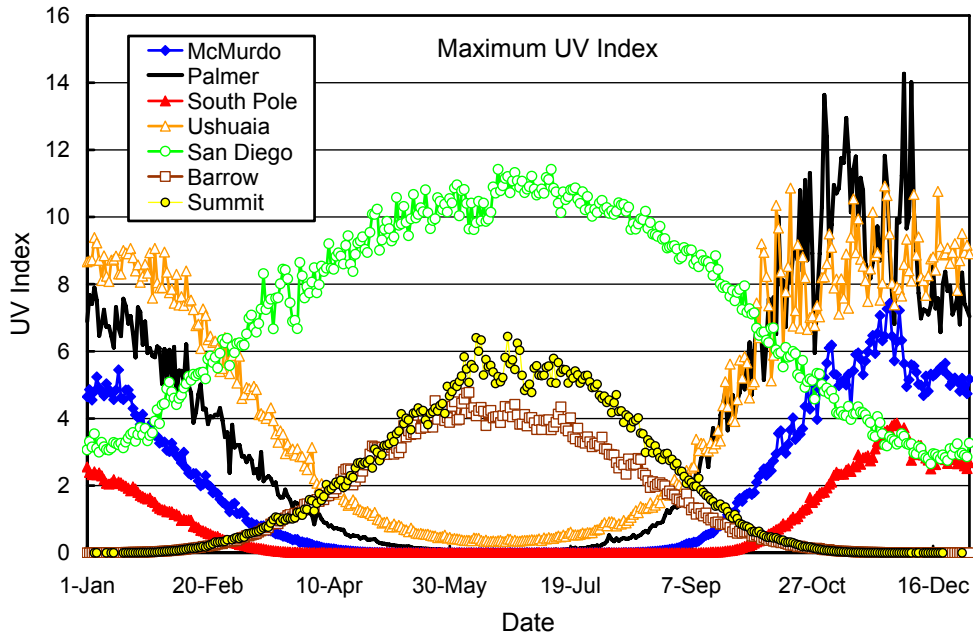
Figure 7.8.3. Comparison of maximum UV Index from all network sites observed at a given day of the year. The data is based on measurements from the years 1991 – 2007 (Summit 2004 – 2007).
