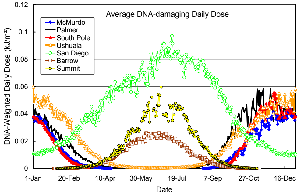
Figure 7.8.5. Comparison of average DNA-weighted daily dose from all network sites. The data is based on average daily doses of the years 1991 – 2007 (Summit 2004 – 2007).
