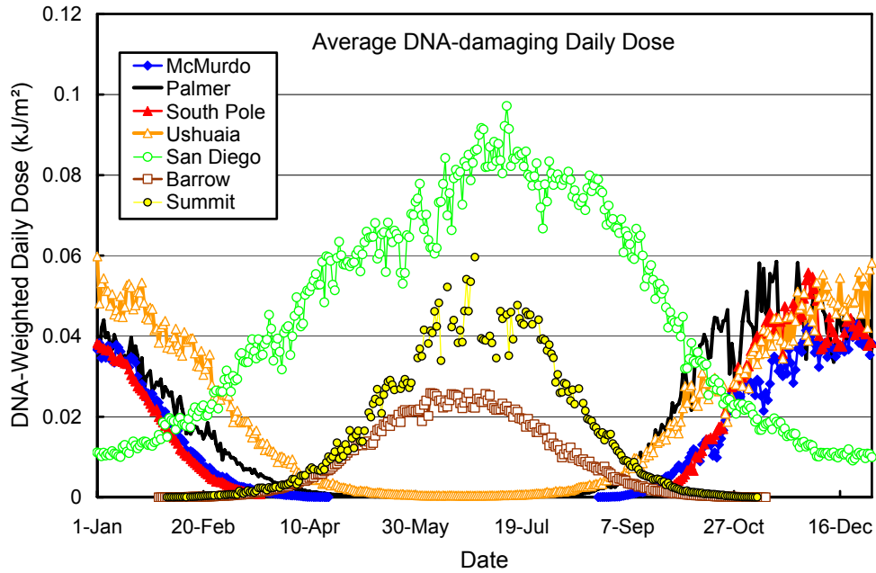
Figure 7.8.5. Comparison of average DNA-weighted daily dose from all network sites. The data is based on average daily doses of the years 1991 – 2007 (Summit 2004 – 2007).
