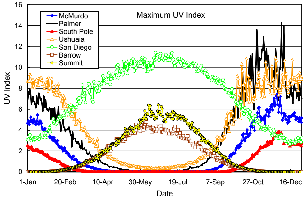
Figure 7.8.3. Comparison of maximum UV Index from all network sites observed at a given day of the year. The data is based on measurements from the years 1991 – 2007 (Summit 2004 – 2007).
