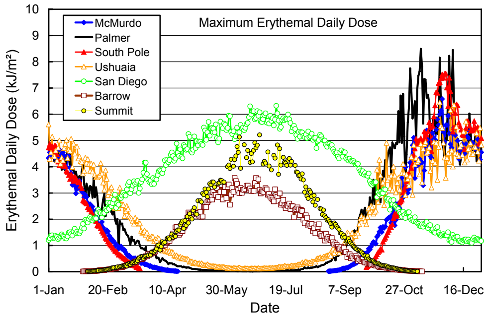
Figure 7.8.4. Comparison of maximum erythemal daily dose from all network sites. The data is based on daily doses of the years 1991 – 2007 (Summit 2004 – 2007).
