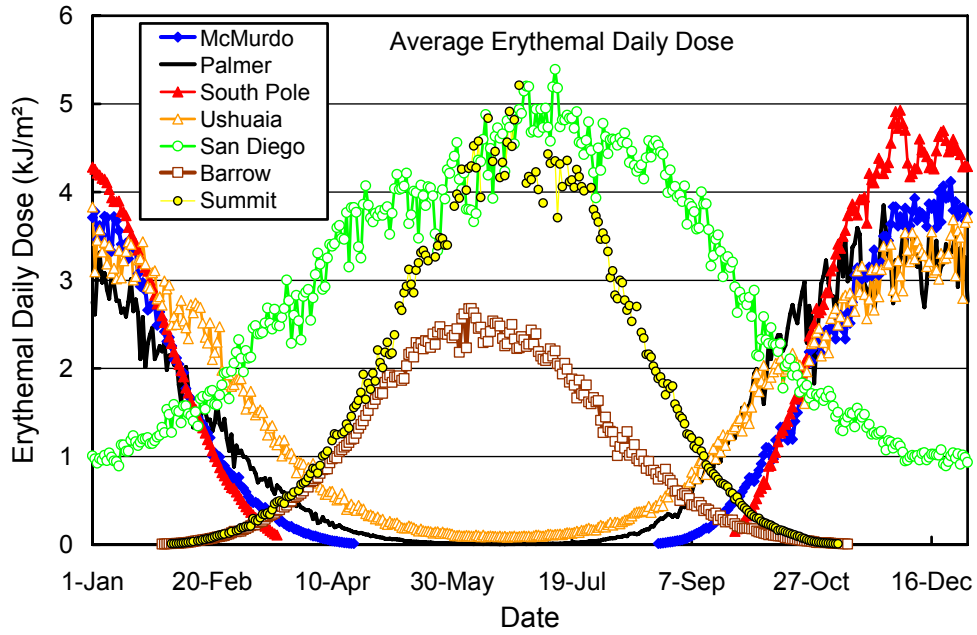
Figure 7.8.1. Comparison of average daily erythemal dose from all network sites. The data is based on average daily doses from the years 1991 – 2007 (Summit 2004 – 2007).
