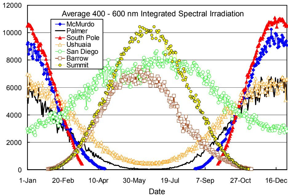
Figure 7.8.6. Comparison of average daily irradiation of the 400-600 nm band from all network sites. The data is based on measurements from the years 1991 – 2007 (Summit 2004 – 2007).
