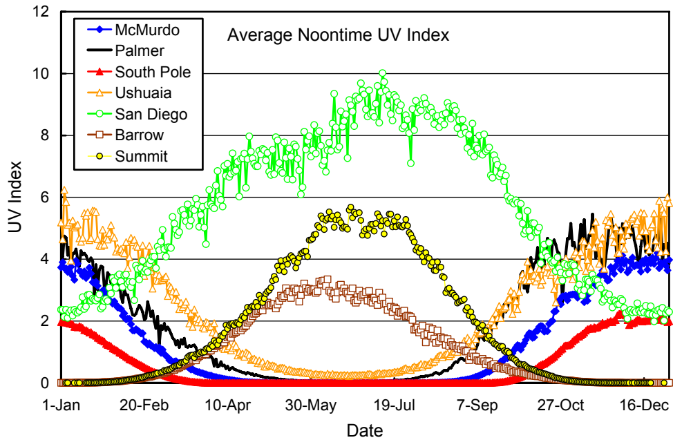
Figure 7.8.2. Comparison of average noontime UV Index from all network sites. Daily measurements from the years 1991 – 2007 (Summit 2004 – 2007) have been averaged.
