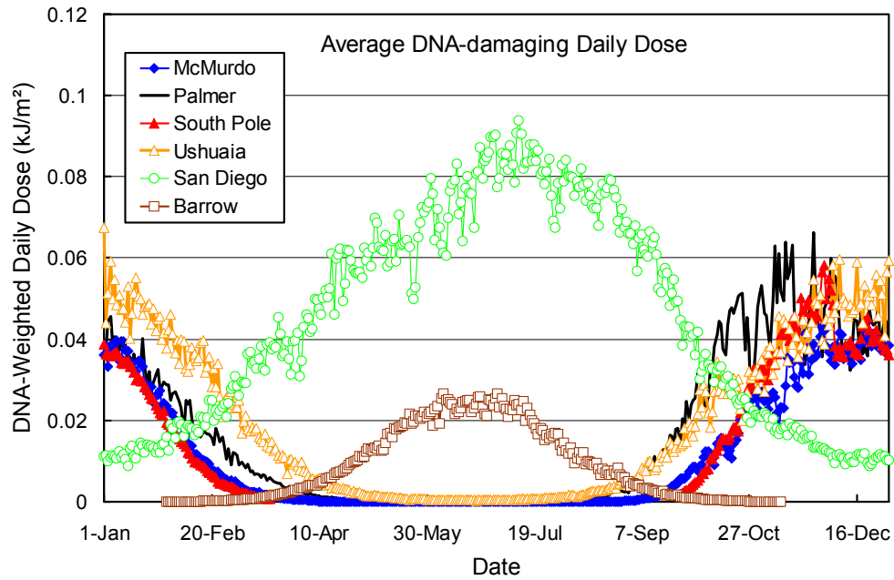
Figure 7.7.5. Comparison of average DNA-weighted daily dose from all network sites. The data is based on average daily doses of the years 1991 – 2004.
