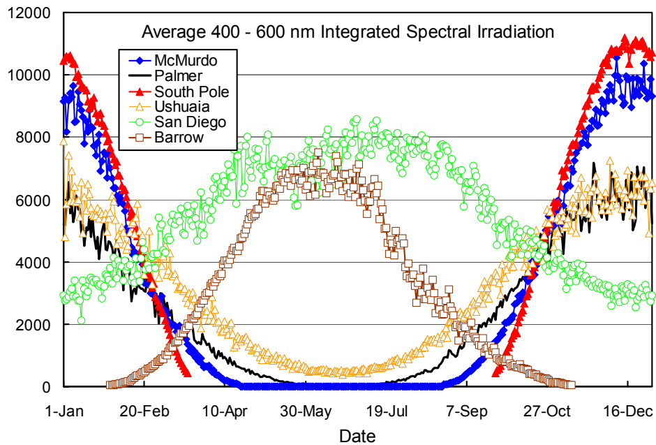
Figure 7.7.6. Comparison of average daily irradiation of the 400-600 nm band from all network sites. The data is based on measurements from the years 1991 – 2004.
