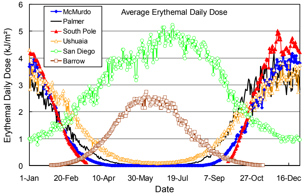
Figure 7.7.1. Comparison of average daily erythemal dose from all network sites. The data is based on average daily doses from the years 1991 – 2004.
