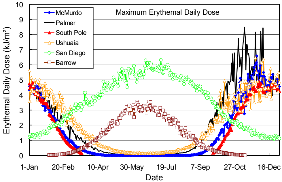
Figure 7.7.4. Comparison of maximum erythemal daily dose from all network sites. The data is based on daily doses of the years 1991 – 2004.
