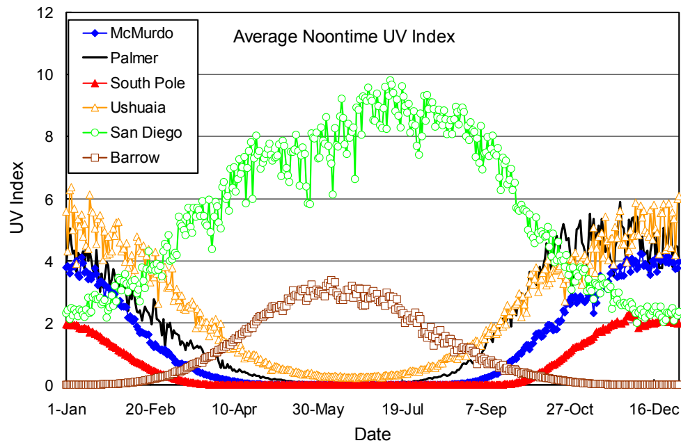
Figure 7.7.2. Comparison of average noontime UV Index from all network sites. Daily measurements from the years 1991 – 2004 have been averaged.
