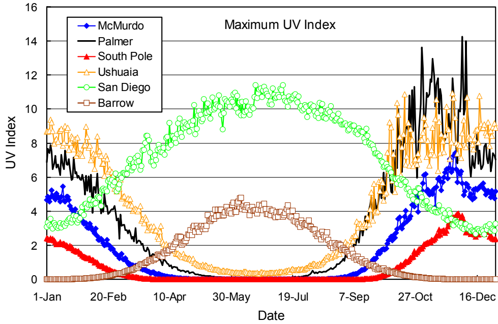
Figure 7.7.3. Comparison of maximum UV Index from all network sites observed at a given day of the year. The data is based on measurements from the years 1991 – 2004.
